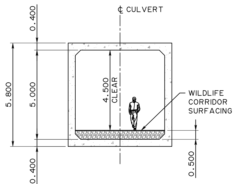
SECTION 1:100
