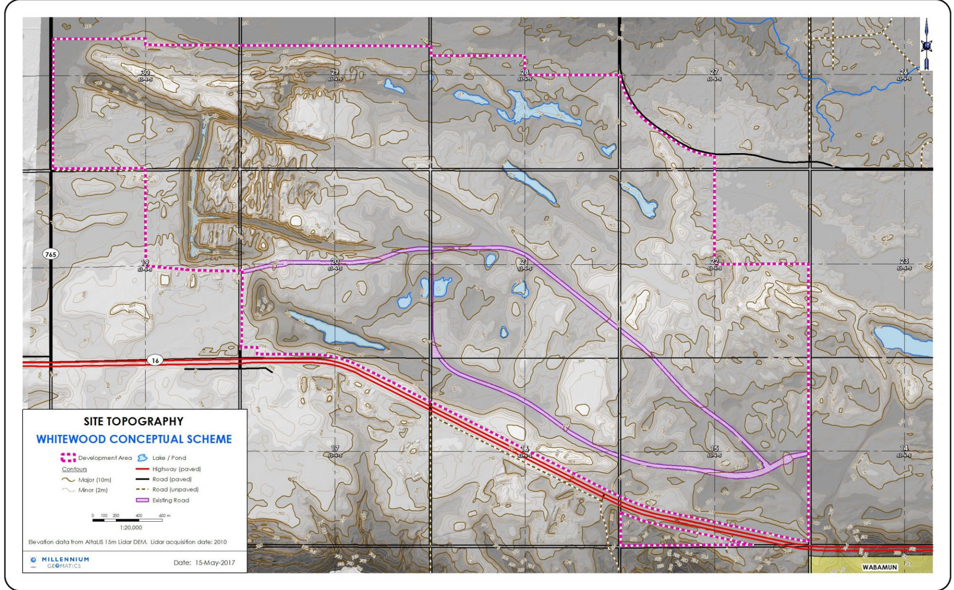
Figure 8: Site Topography
